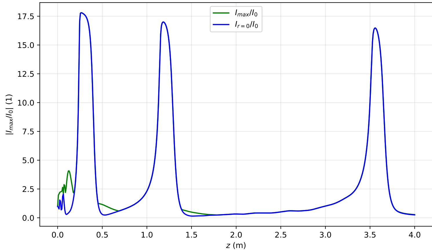
I_{max}(x = 0, y = 0, z)/I_0 , \text{Pin}=4.0\text{Pcr} , artificial time
